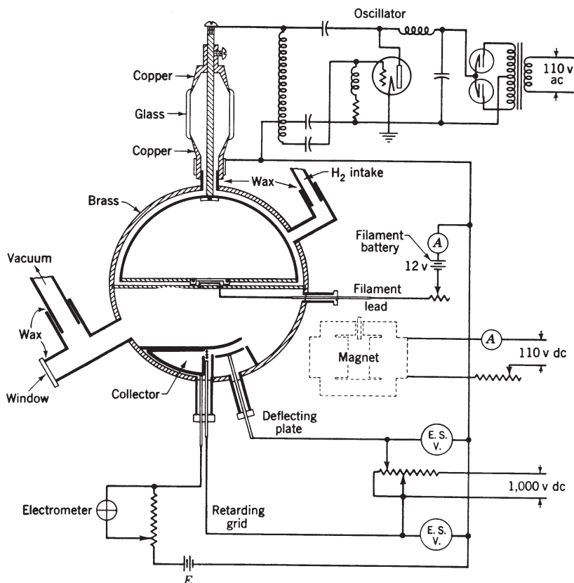
Figure 5.3. Livingston's cyclotron, with its charging circuit. Livingston, The Production of High Velocity Hydrogen Ions Without the Use of High Voltages, PhD thesis, University of California, Berkeley, 14 April 1931, figure 3.
